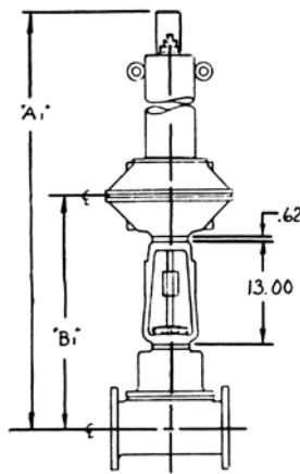
Yoke Mounted
