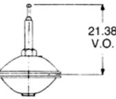
Adjustable Opening and Adjustable Travel Stop
