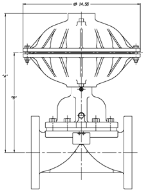
Close Coupled
