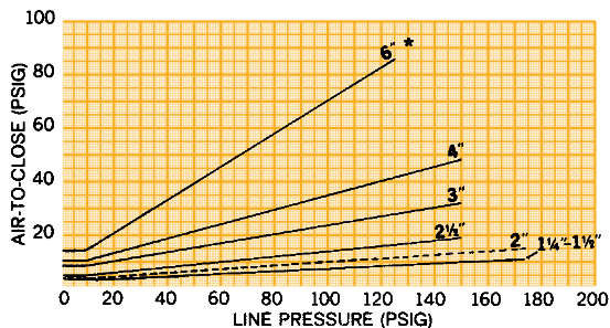
Chart E No. 50 ACTUATOR with ELASTOMER Diaphragm
