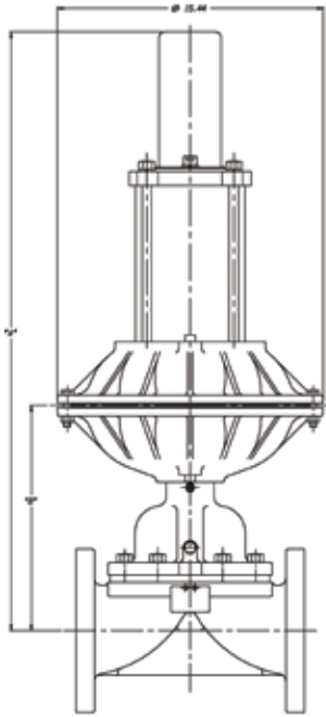
Close Coupled
