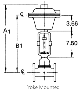
Yoke Mounted
