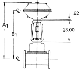
Yoke Mounted
