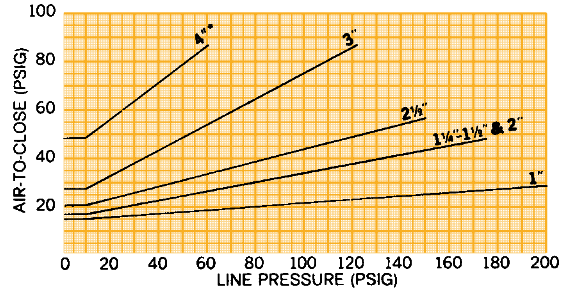
Chart D No. 25 ACTUATOR with PTFE PLASTIC Diaphragm
