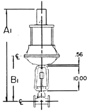
Yoke Mounted
