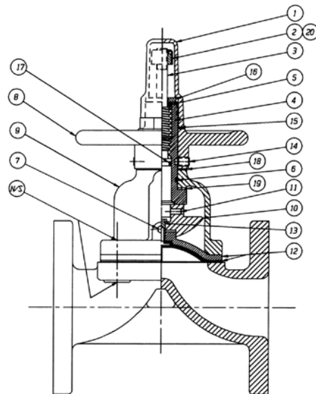
903 BONNET ½" Through 4" Standard Consult Factory for 6"
