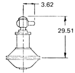
Positioner (Moore & Conoflow)
