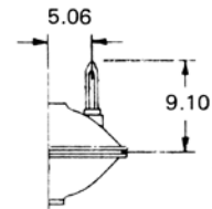
Position Indicator
