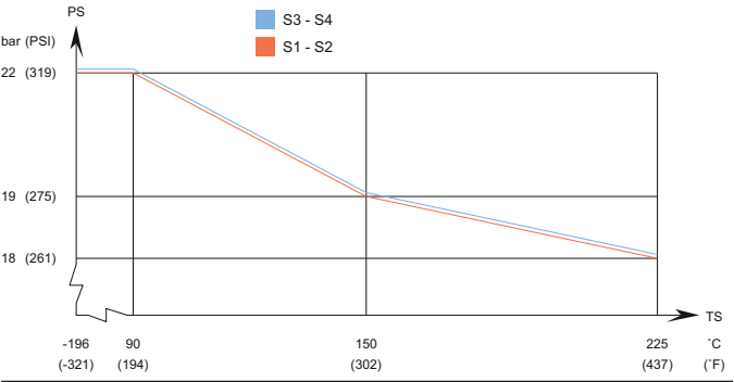
DOC410 – PED approval pressure/temperature graph
