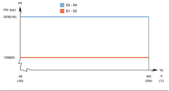
AXP82 – UL approval pressure/temperature graph
