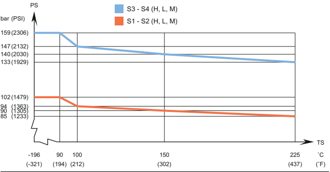
AXP82 – UL approval pressure/temperature graph
